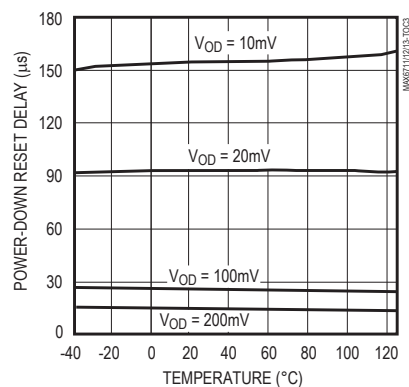
MAX671_L/M POWER-DOWN RESET DELAY vs. TEMPERATURE
